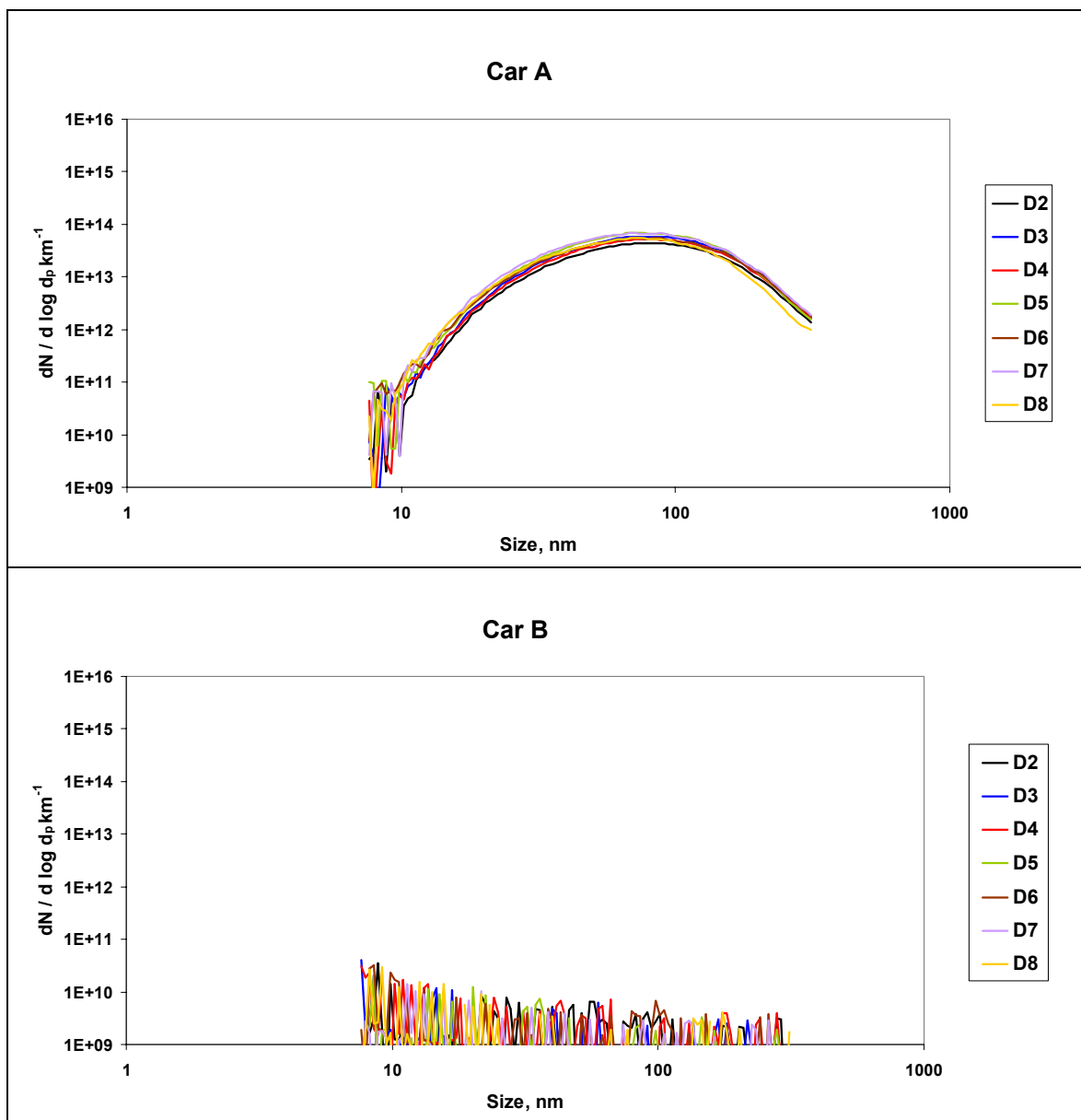
Figure 29 SMPS Distributions at 50km/h
