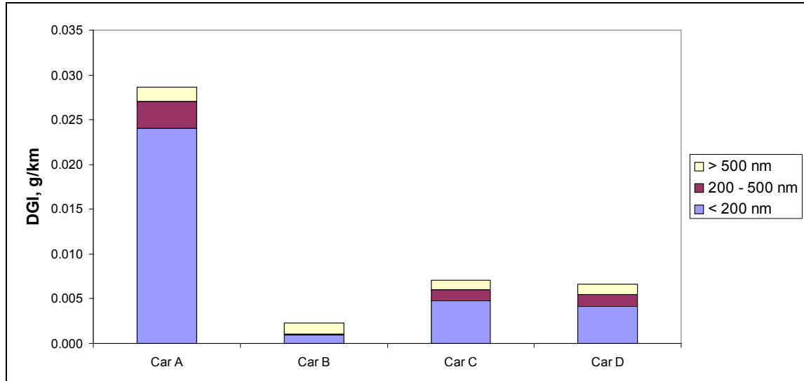
Figure 21 DGI data (arithmetic means) over NEDC
