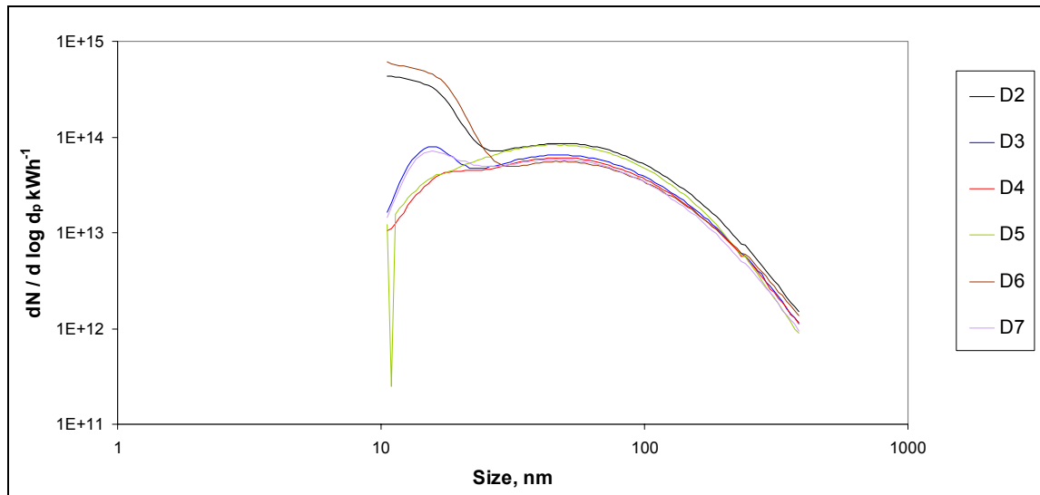
Figure 10 ESC: SMPS distribution for each fuel in the Euro-3 engine
