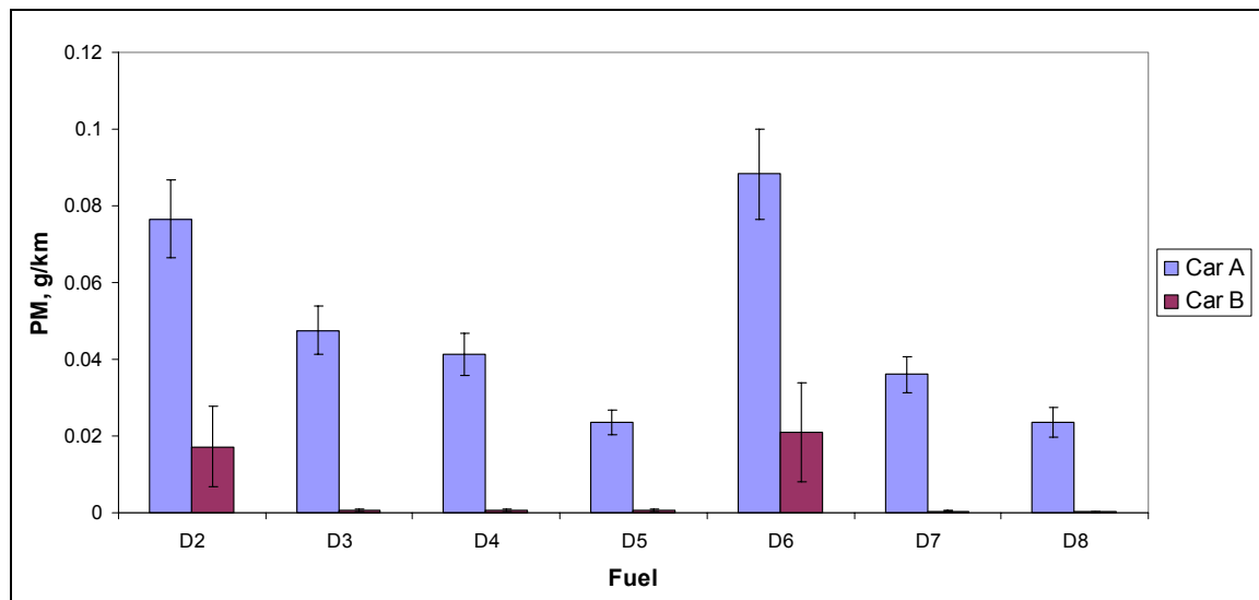
Figure 20 PM emissions at 120 km/h
