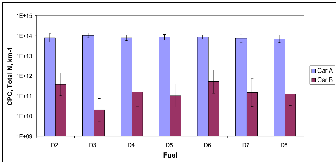
Figure 25 CPC total particle count - NEDC
