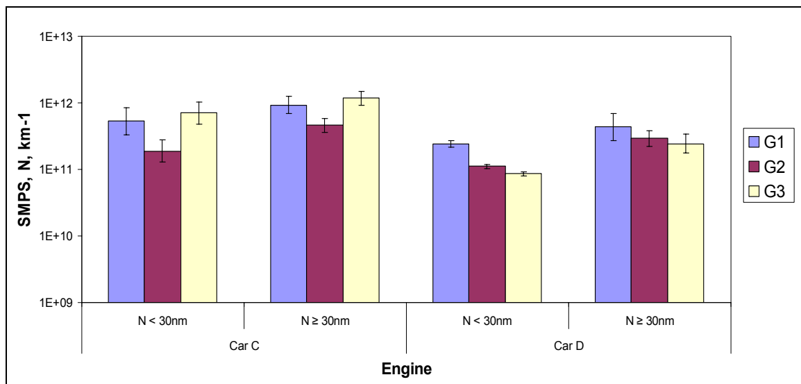
Figure 40 SMPS particle numbers, <30nm and >30nm: 120 km/h data
