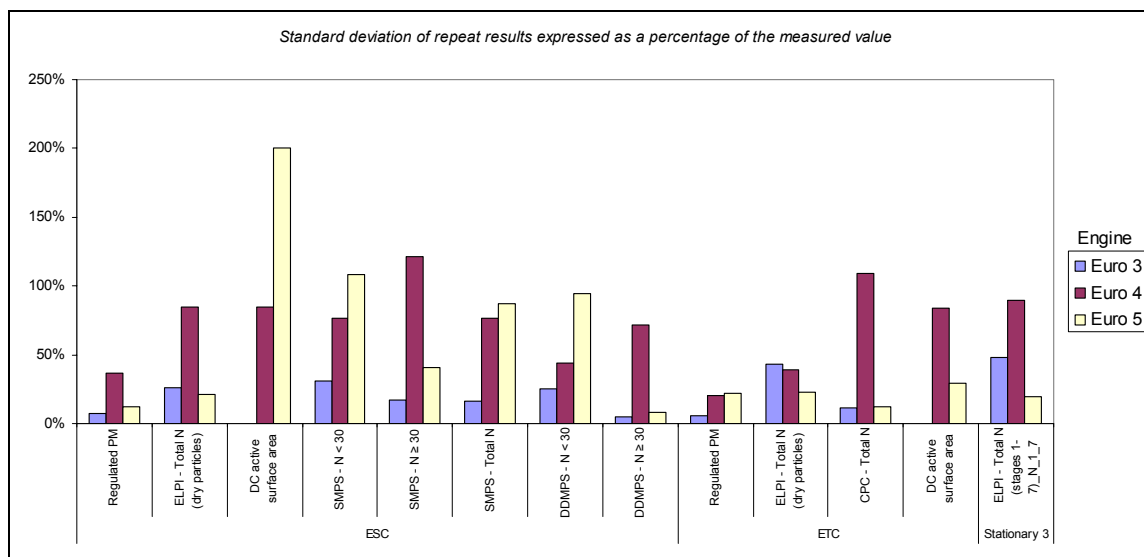
Figure 43 Precision of heavy-duty particle measurements
