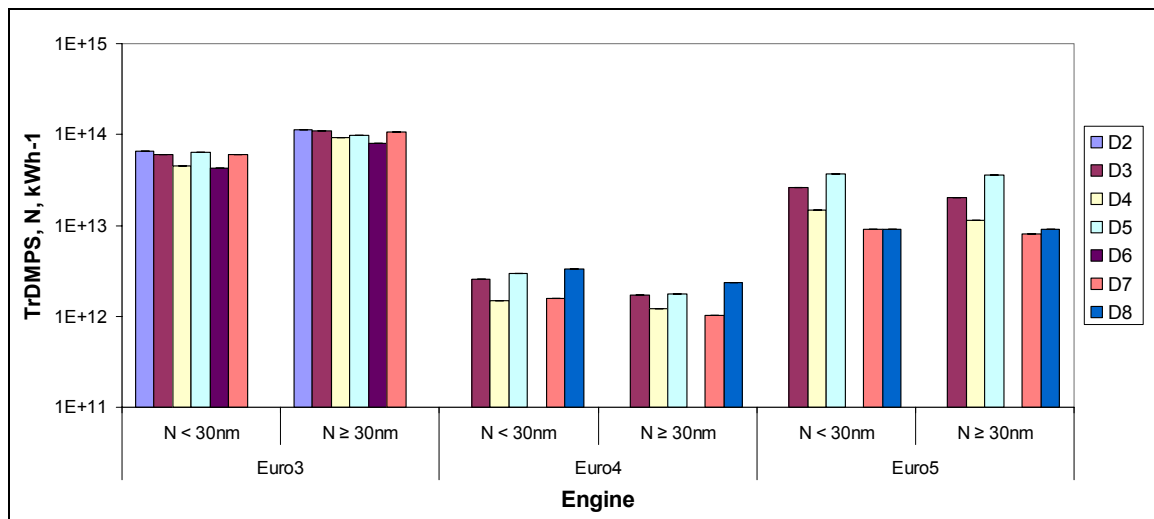
Figure 15 ETC total particle count by TrDMPS: particles <30nm and >30nm
