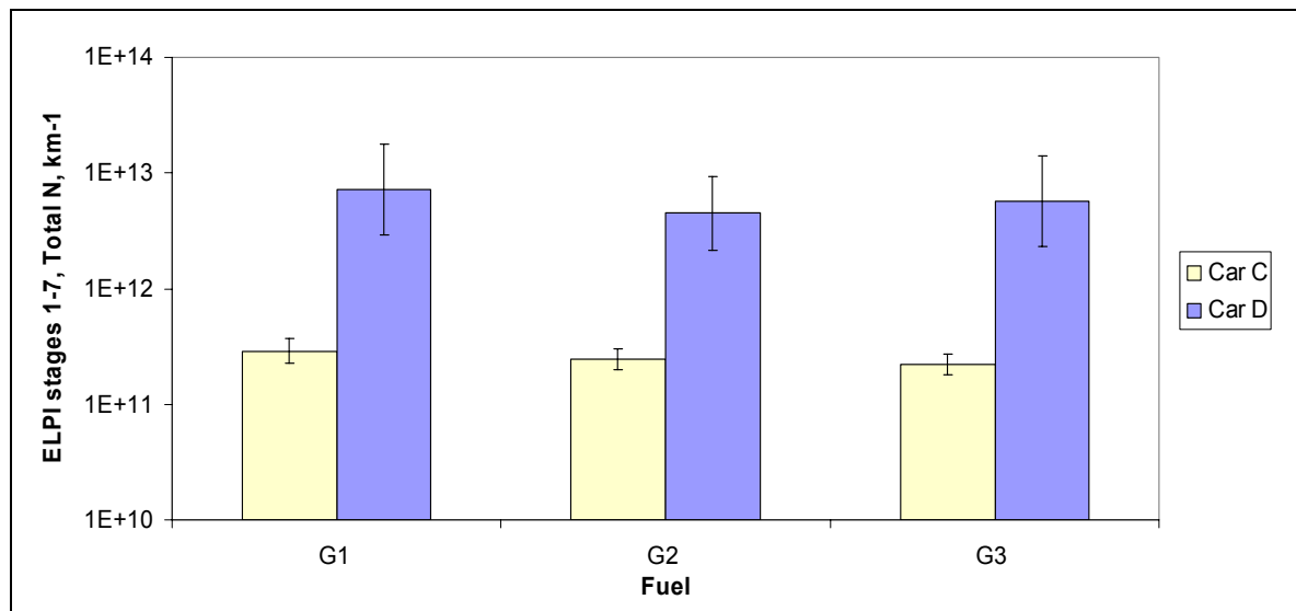
Figure 36 Total count ELPI stages 1-7 (30-1000nm) + thermodenuder, 50km/h
