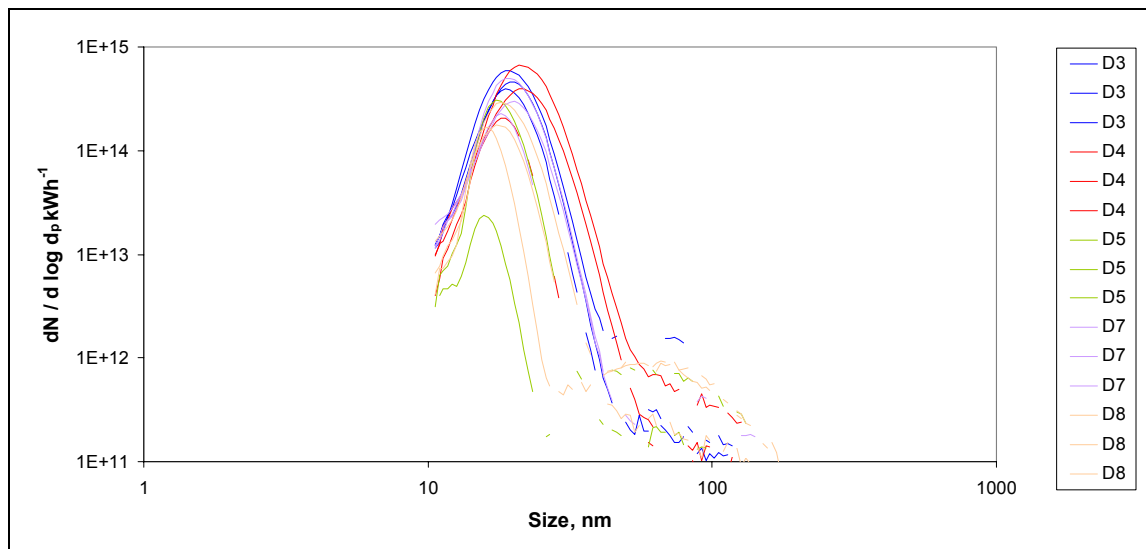
Figure 11 ESC: SMPS distribution for each fuel in the Euro-4 engine
