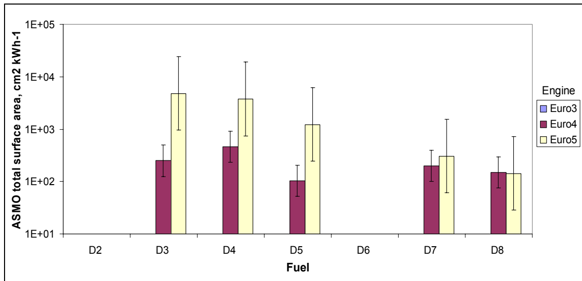
Figure 17 ASMO total surface area - ETC
