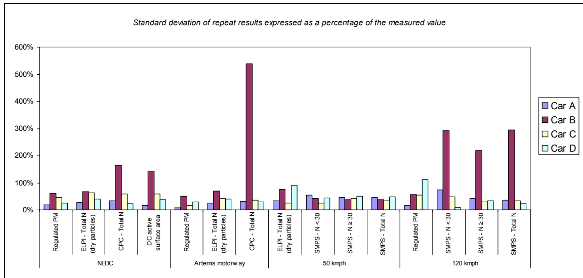
Figure 44 Precision of light-duty particle measurements
