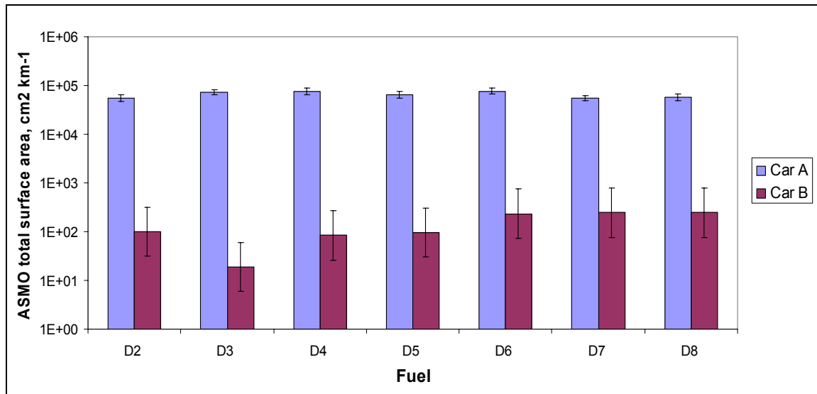
Figure 32 ASMO total surface area - NEDC
