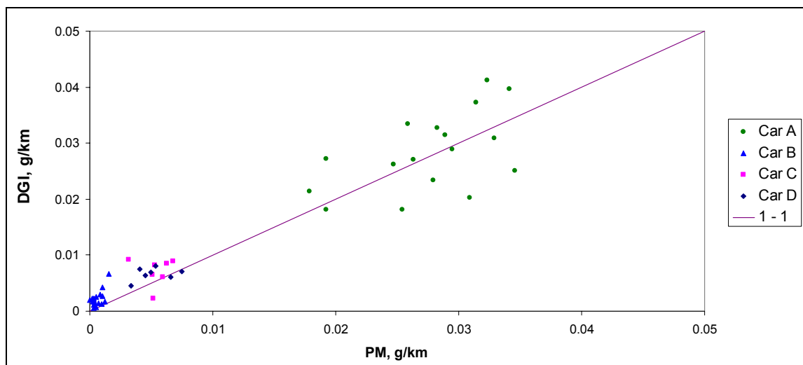
Figure 22 DGI versus regulated PM over NEDC
