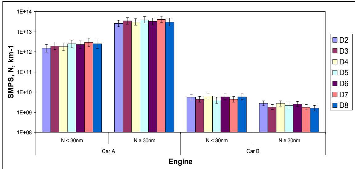
Figure 27 50km/h total particle count by SMPS: particles <30nm and >30nm
