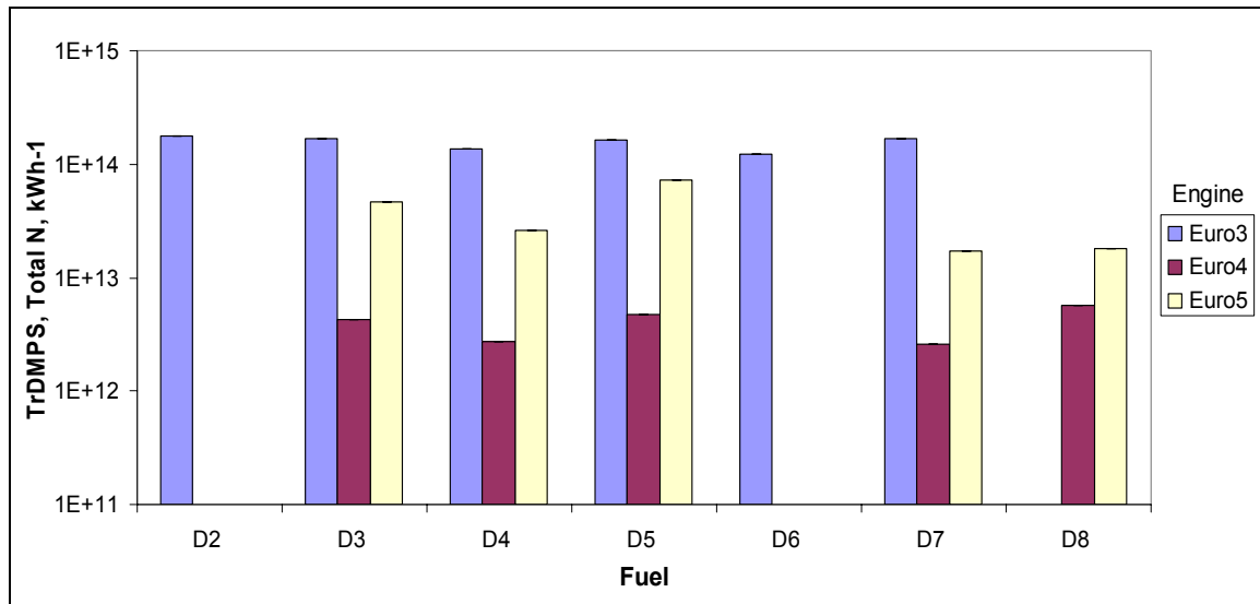
Figure 14 ETC total particle count by TrDMPS
