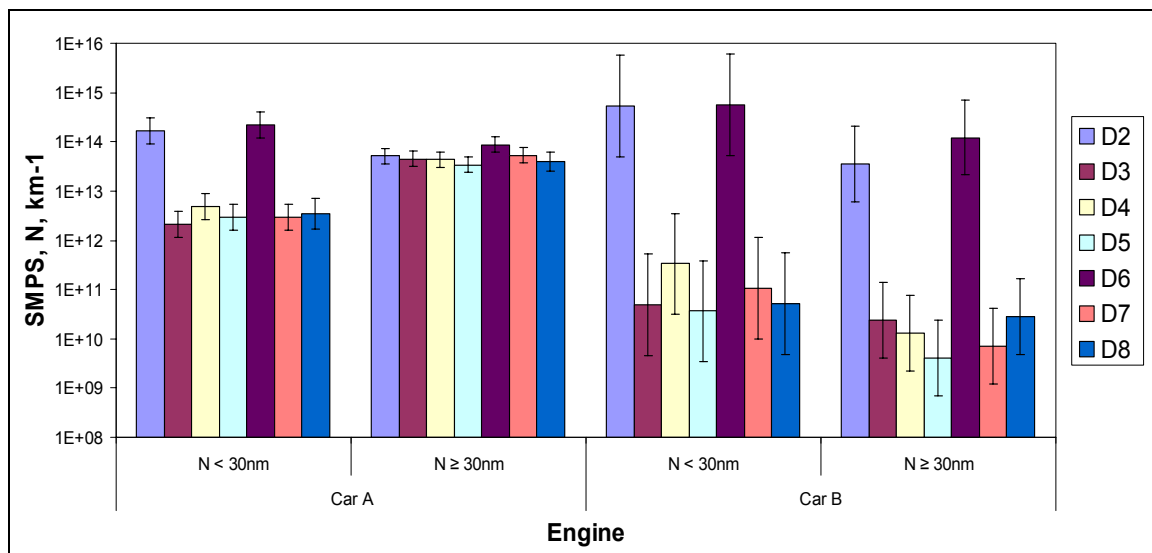
Figure 28 120km/h total particle count by SMPS: particles <30nm and >30nm
