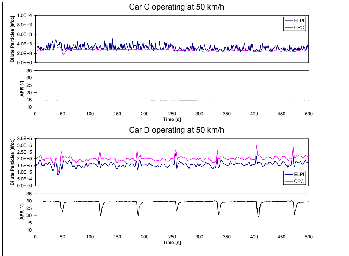
Figure 41 Typical AFR and Particle number traces for the two gasoline cars operating at 50 km/h and 120 km/h
