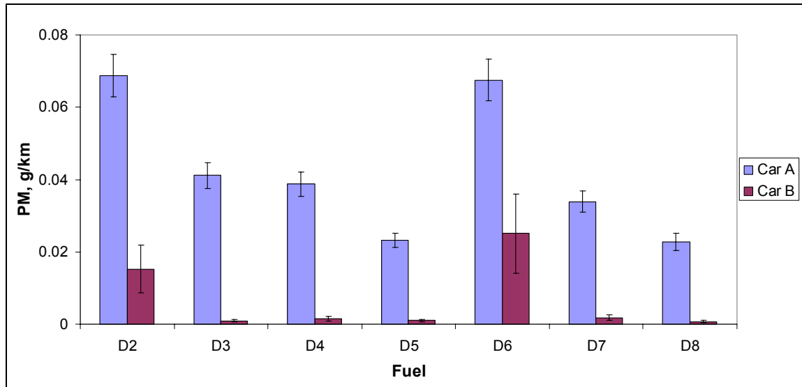
Figure 19 PM emissions - Artemis motorway cycle
