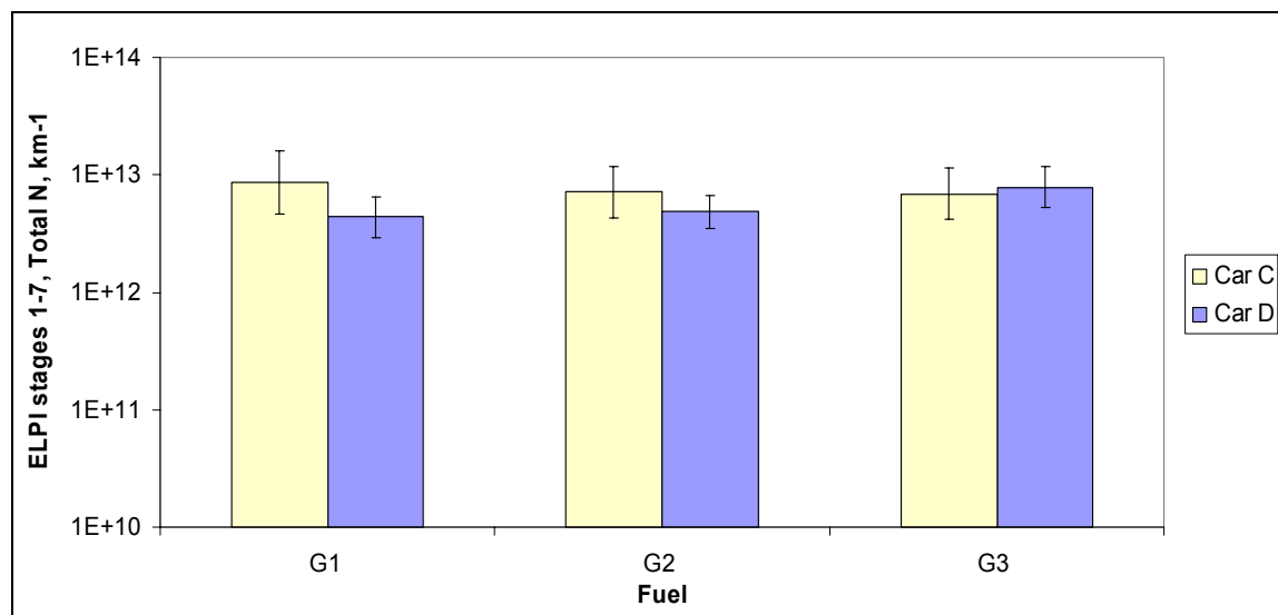
Figure 35 Total count ELPI stages 1-7 (30-1000nm) + thermodenuder, NEDC
