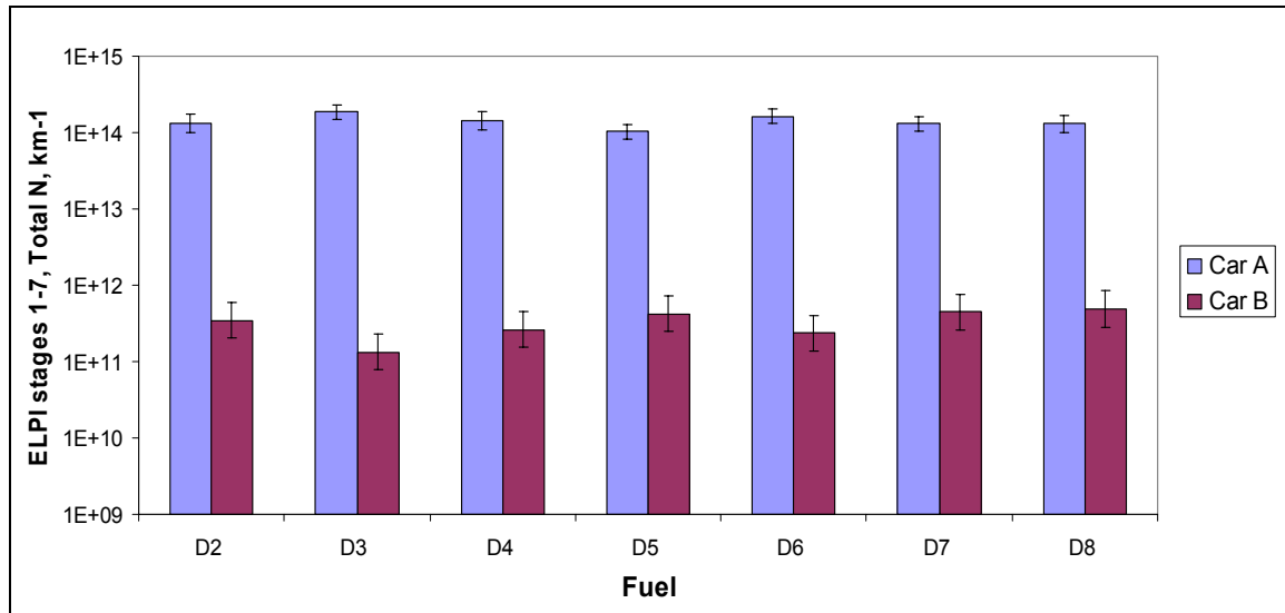
Figure 23 Total count ELPI stages 1-7 (30-1000nm) + thermodenuder, NEDC
