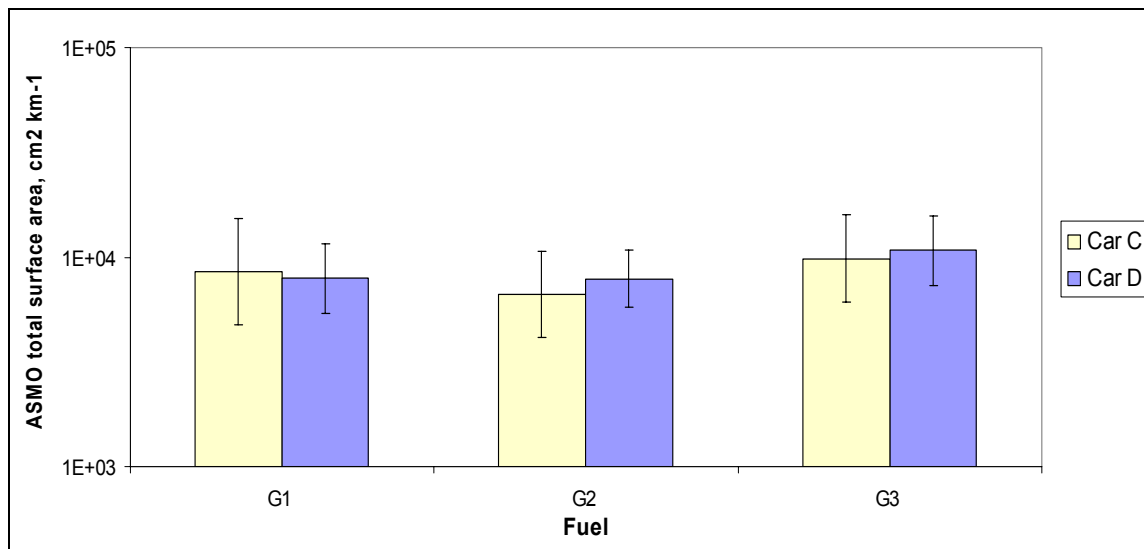
Figure 42 ASMO total surface area - NEDC
