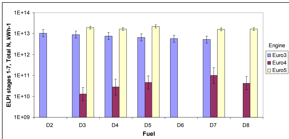
Figure 6 Total count ELPI stages 1-7 (30-1000nm) + thermodenuder, SS3
