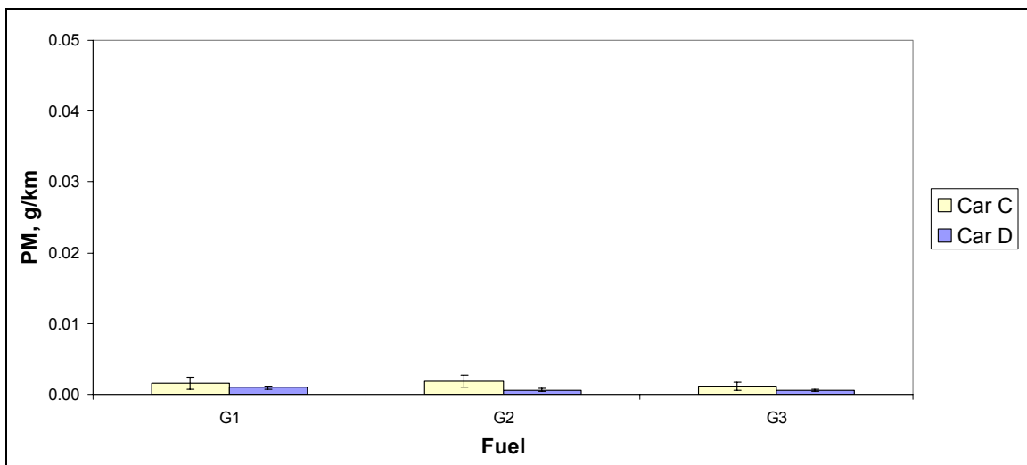
Figure 34 Particulate mass - Artemis motorway cycle
