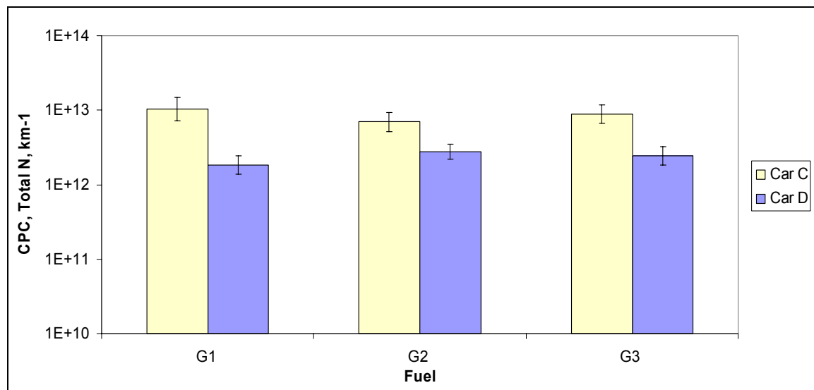
Figure 38 CPC total particle count - Artemis motorway cycle
