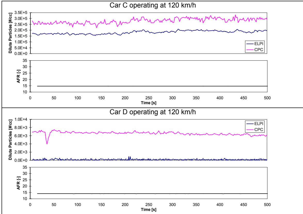
Figure 41 demonstrates that the two vehicles have different operating strategies.
