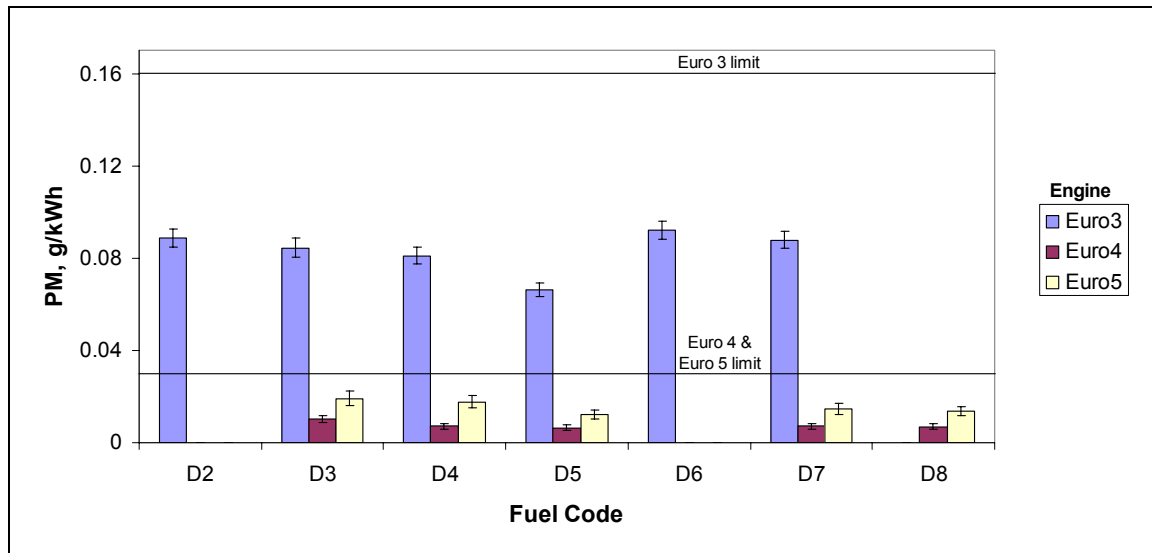
Figure 3 PM emissions - ETC
