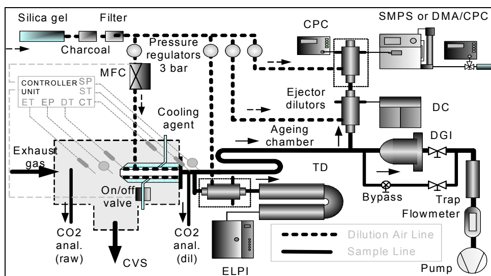
Figure 1 Diagram of 'PARTICULATES' Measuring System
