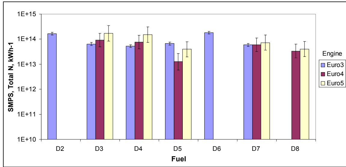
Figure 7 ESC Total particle count by SMPS
