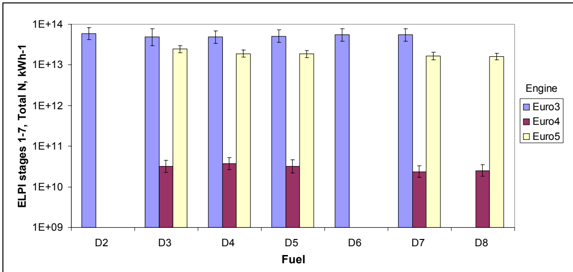
Figure 5 Total count ELPI stages 1-7 (30-1000nm) + thermodenuder, ETC
