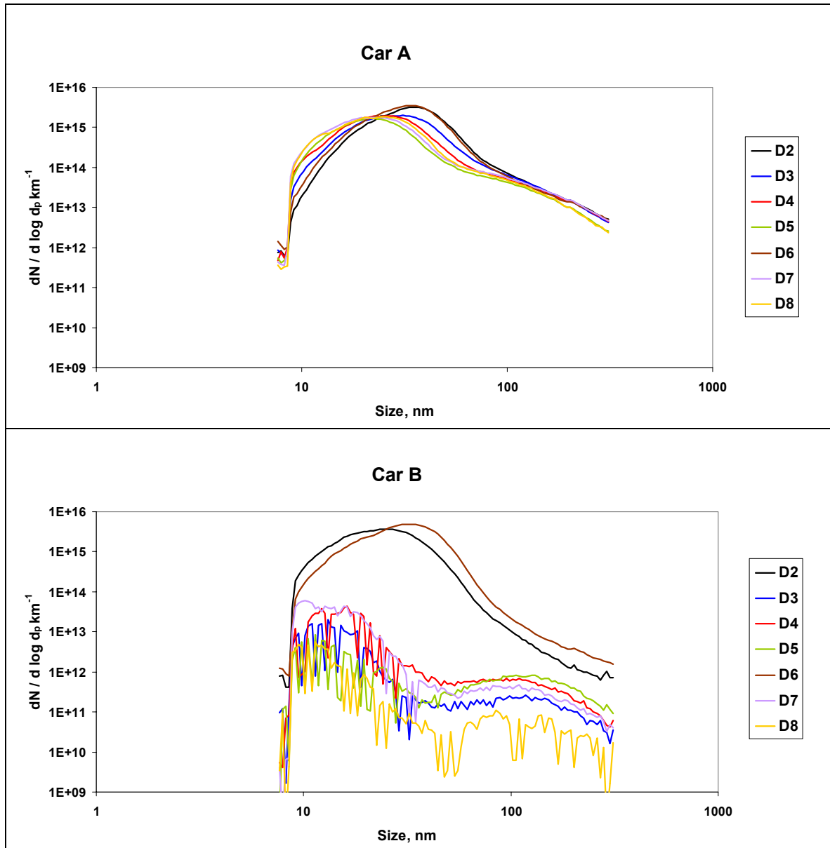
Figure 31 SMPS Distributions at 50km/h - high load
