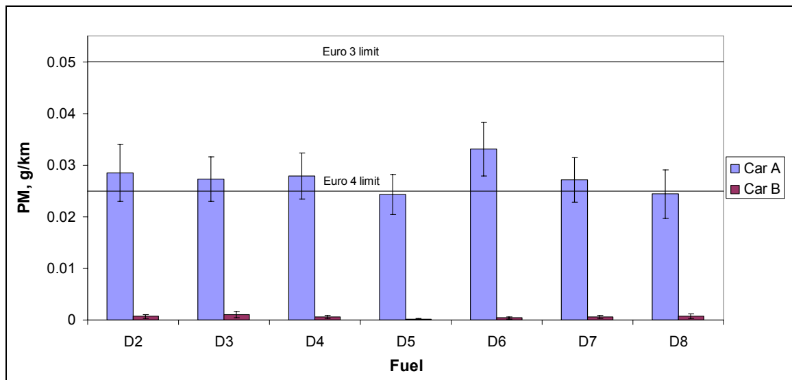
Figure 18 Regulated PM emissions - NEDC
