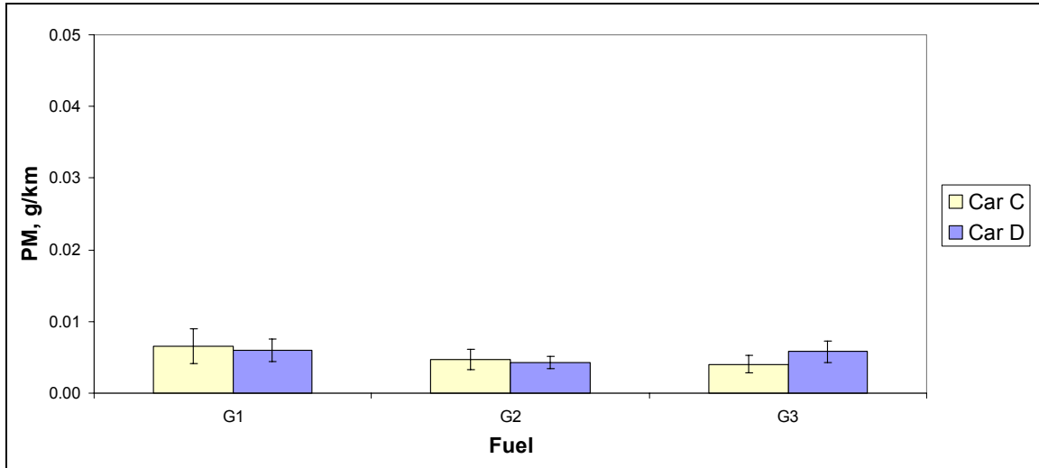
Figure 33 Particulate mass - NEDC
