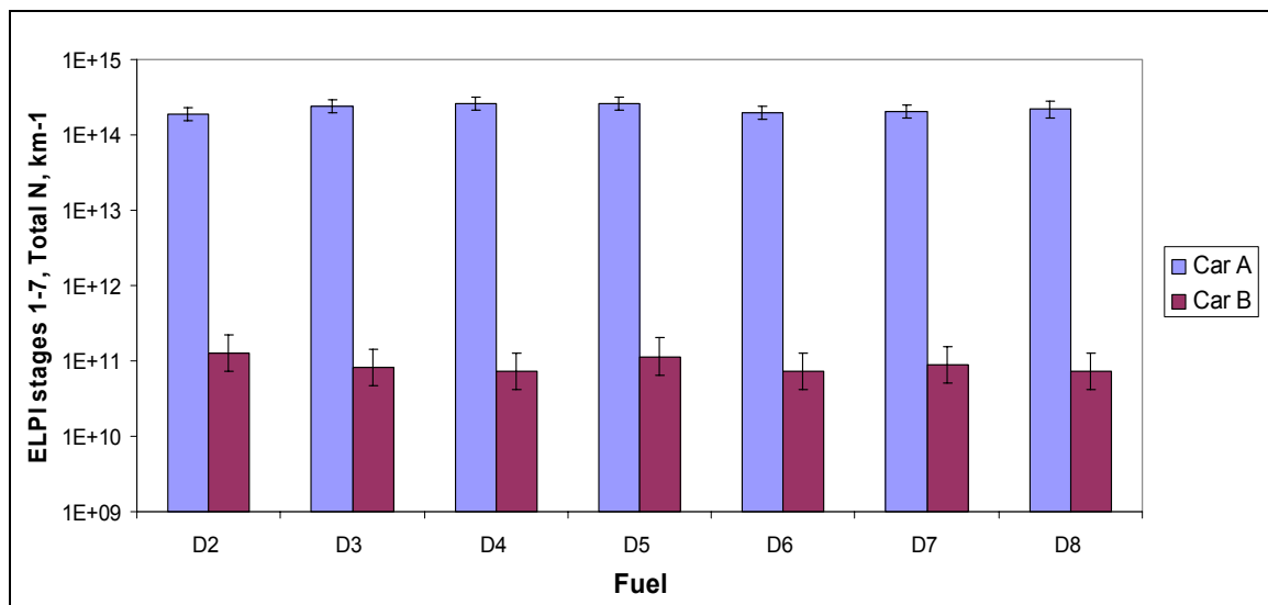
Figure 24 Total count ELPI stages 1-7 (30-1000nm) + thermodenuder, Artemis motorway cycle
