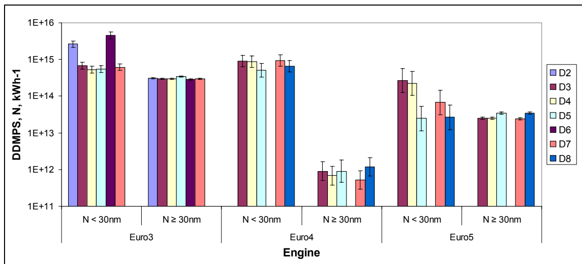
Figure 9 ESC total particle count by DDMPs: particles <30nm and >30nm
