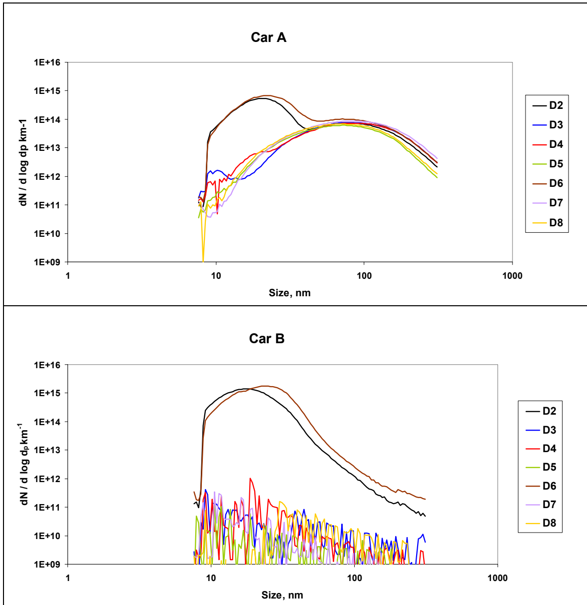
Figure 30 SMPS Distributions at 120km/h
