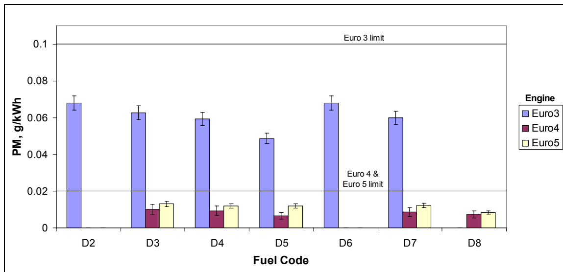
Figure 2 PM emissions - ESC
