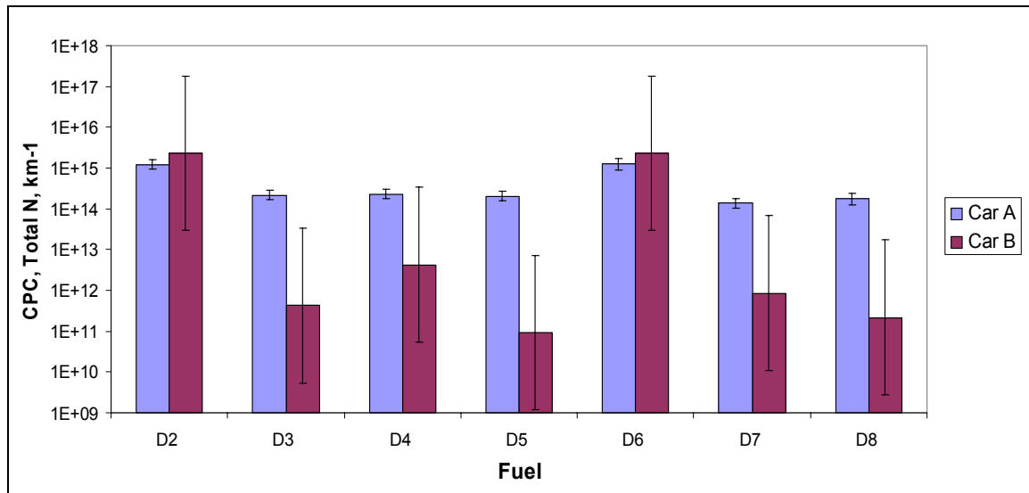
Figure 26 CPC total particle count - Artemis motorway cycle
