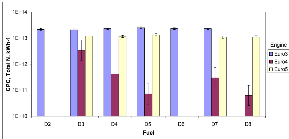
Figure 13 ETC total particle count by CPC
